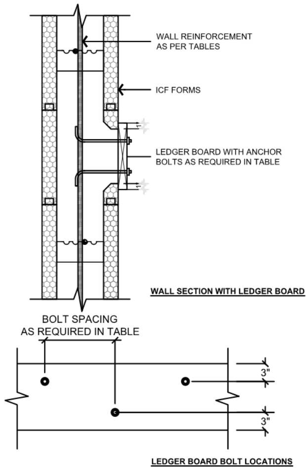
Detail C. 1. Wood Ledger Connection
